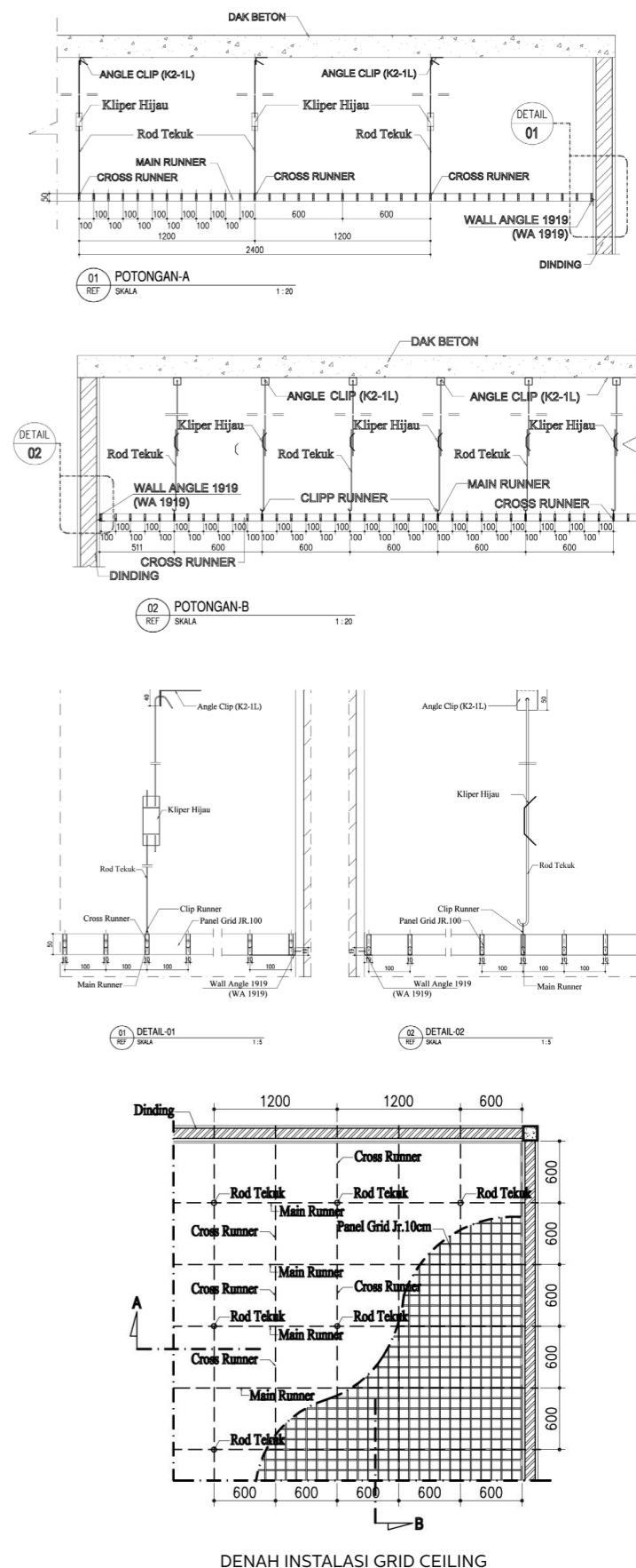
DENAH INSTALASI GRID CEILING
