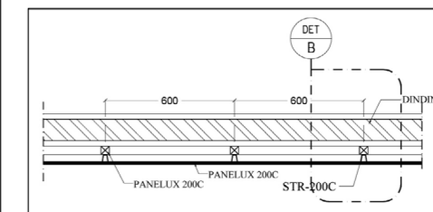
POTONGAN-B SKALA 1:5
